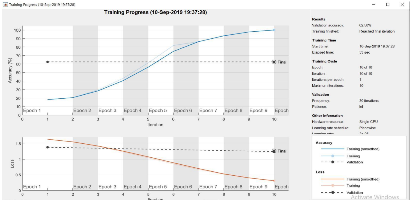
Figure 21. Training Progress
