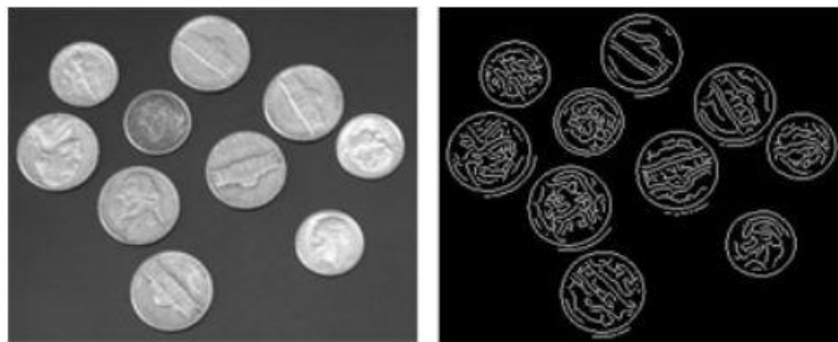
Figure 4. Canny Edge Detector
